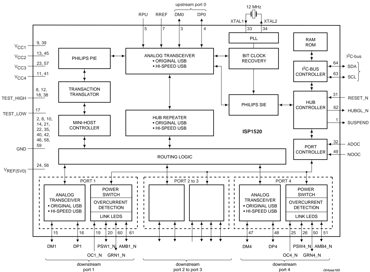
Fig 1. Block diagram.
